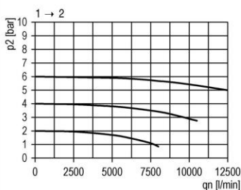
flow characteristic
